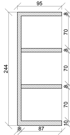
SECTION B-B
