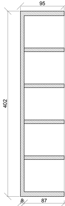
SECTION B-B
