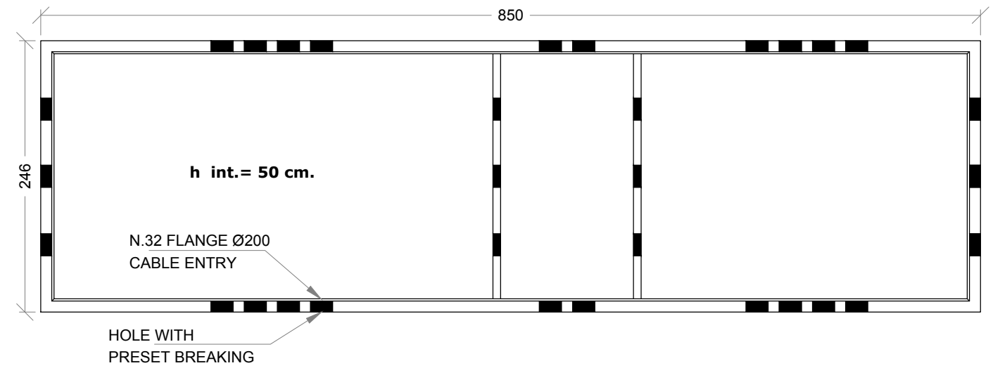
FOUNDATION TANK
